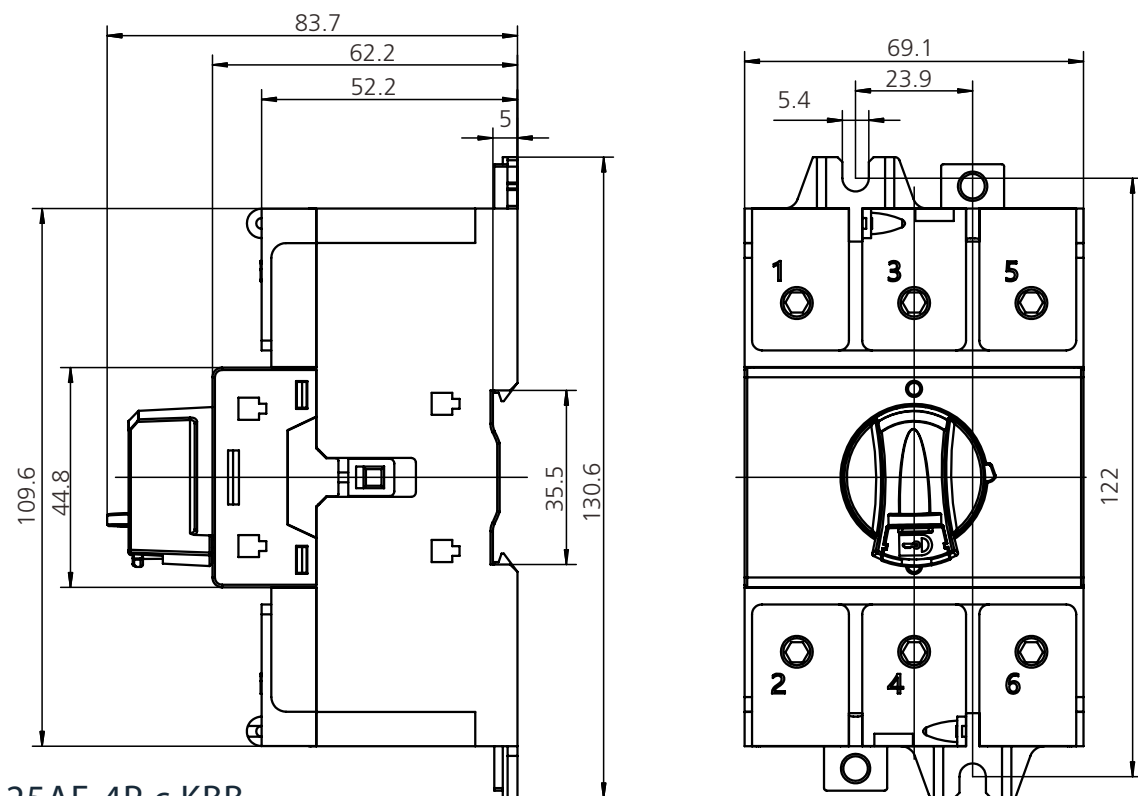
125AF-4P с KBB
